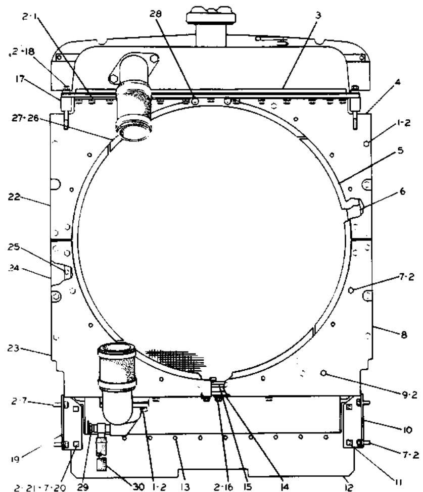
2P8182 RADIATOR GROUP - Rear View
