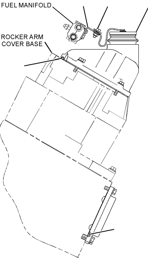
FRONT VIEW OF ENGINE
