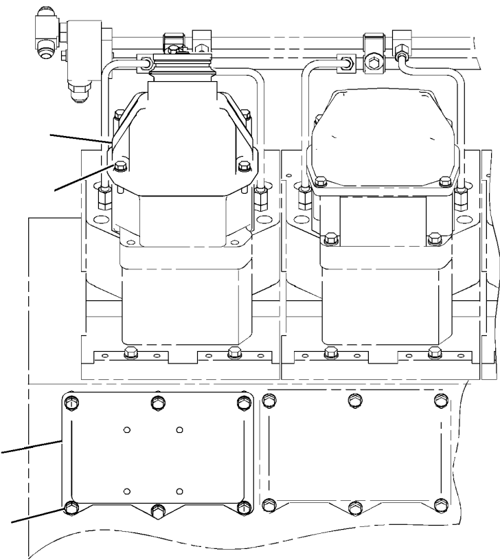
LEFT SIDE VIEW OF ENGINE
