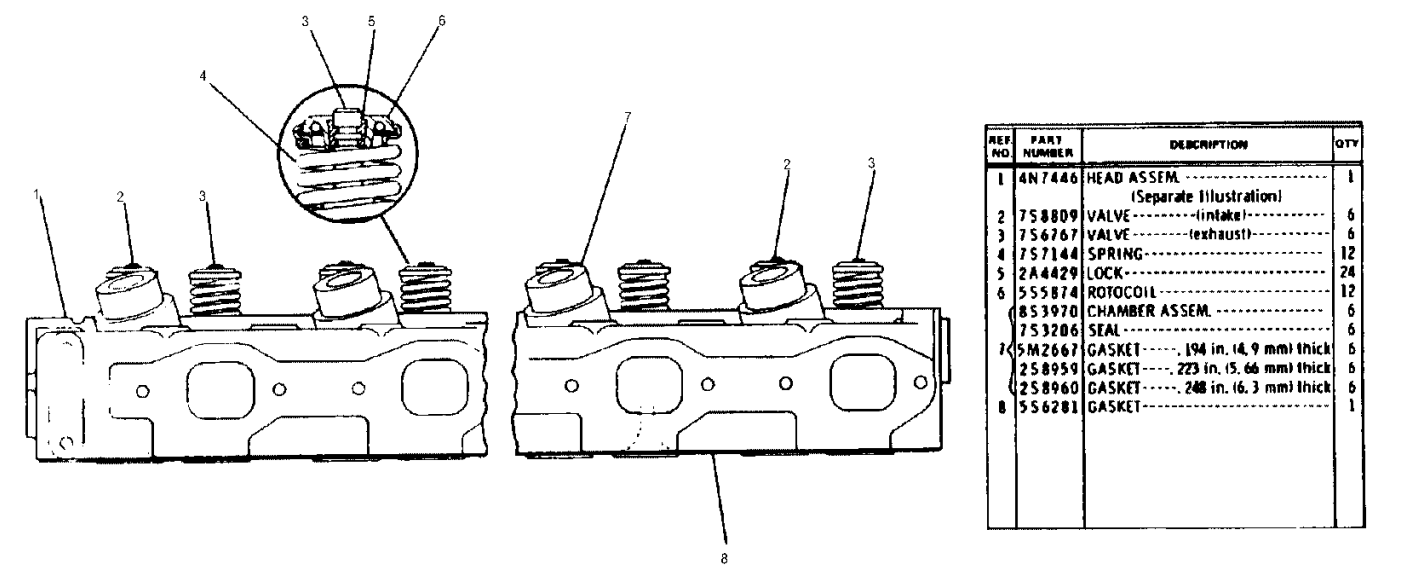
Drawing 1 of 1
