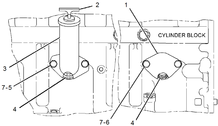
RIGHT SIDE VIEW OF ENGINE
