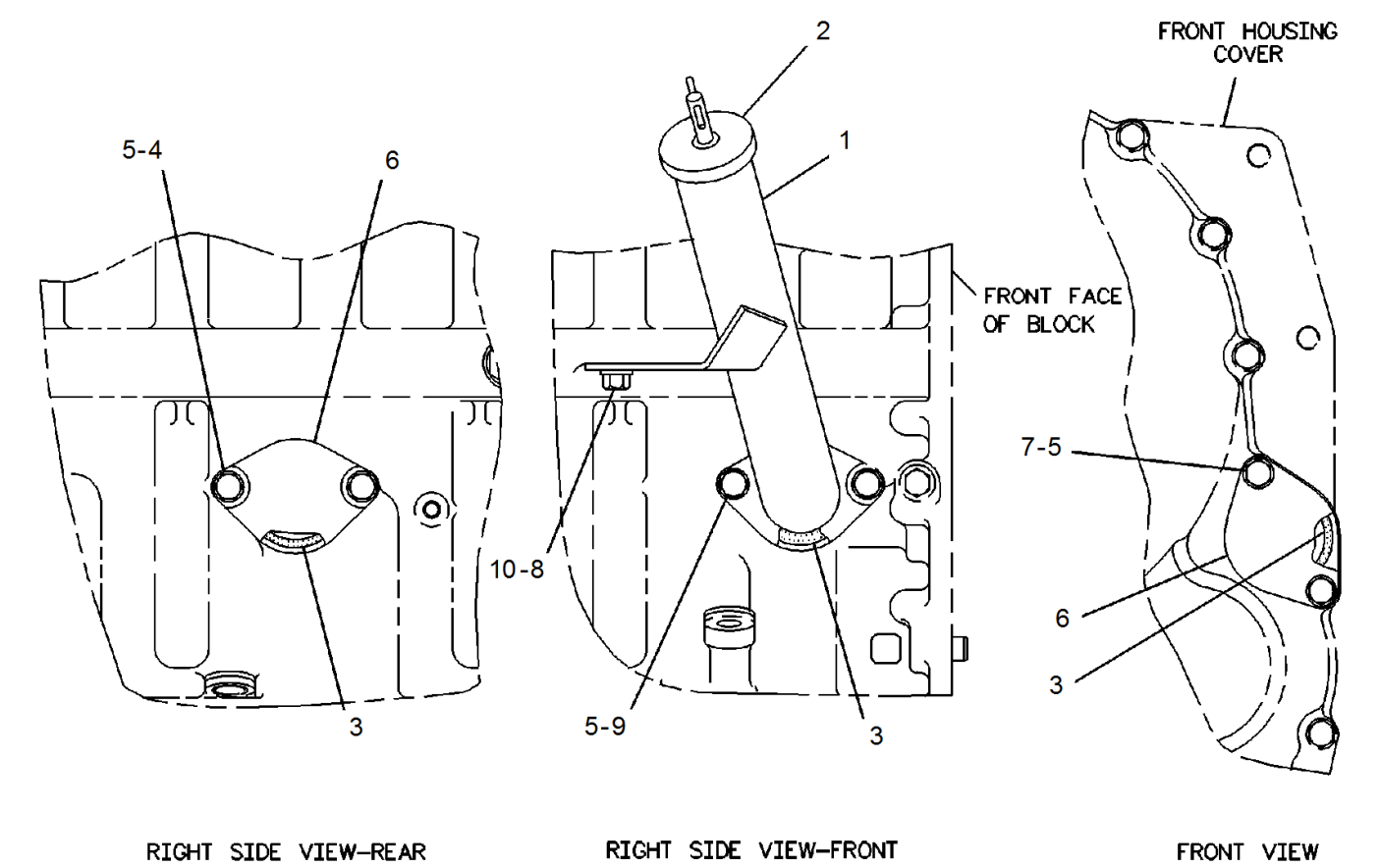
Drawing 1 of 1
