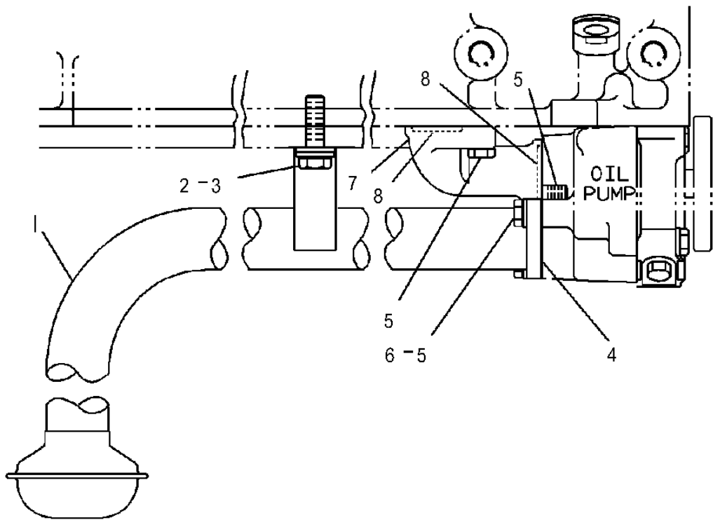
SIDE VIEW
