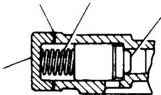
VIEW A - A
