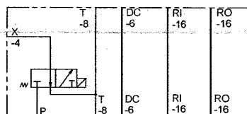
HYDRAULIC CHART
