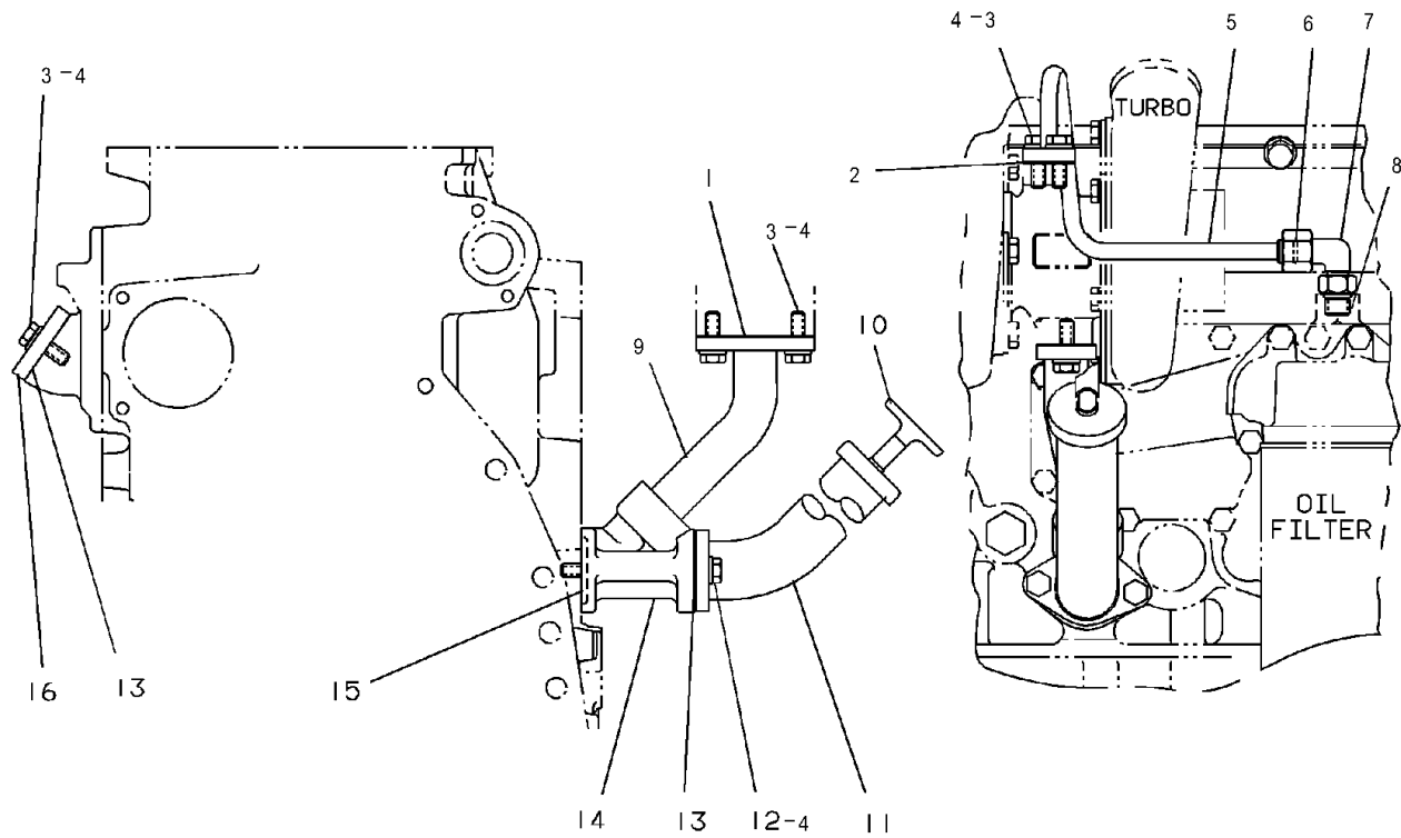
REAR VIEW
