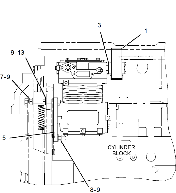
LEFT SIDE VIEW OF ENGINE
