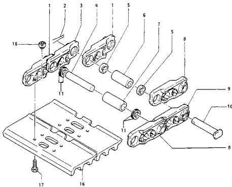
TRACK - 600mm (23-5/8") TRIPLE GROUSER SHOES An Attachment
