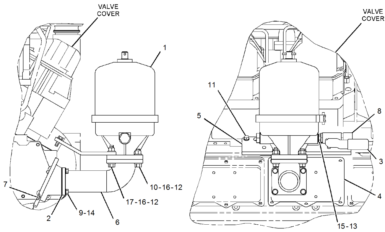
FRONT VIEW OF ENGINE LEFT SIDE VIEW OF ENGINE
