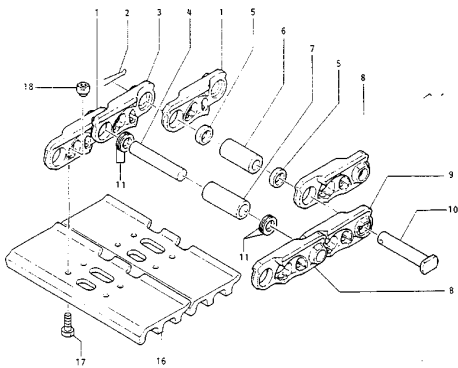
TRACK - 500mm (19-5/8") TRIPLE GROUSER SHOES
