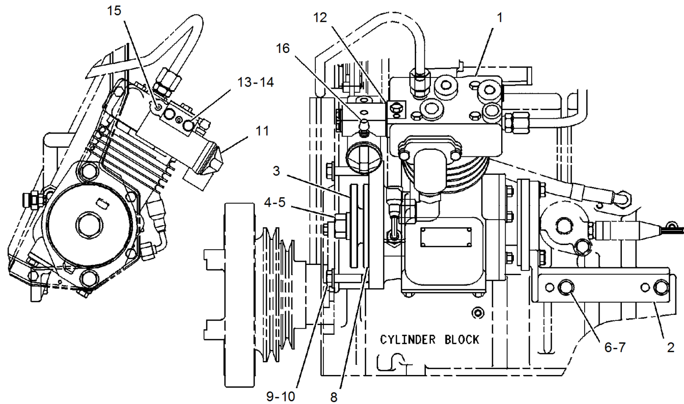
FRONT VIEW
