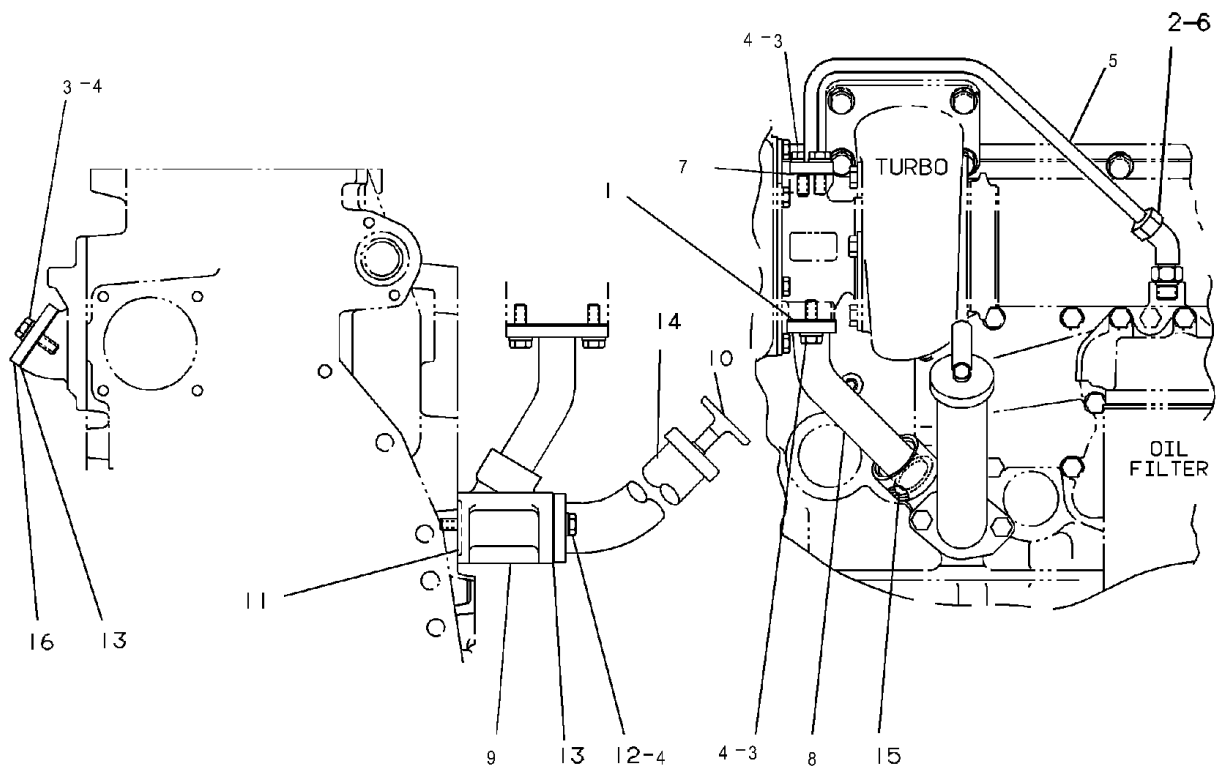
REAR VIEW
