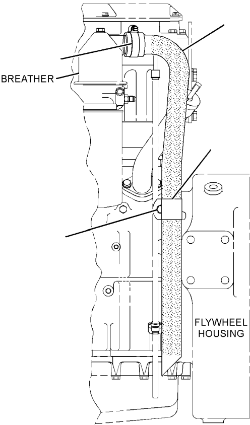
LEFT SIDE VIEW OF ENGINE
