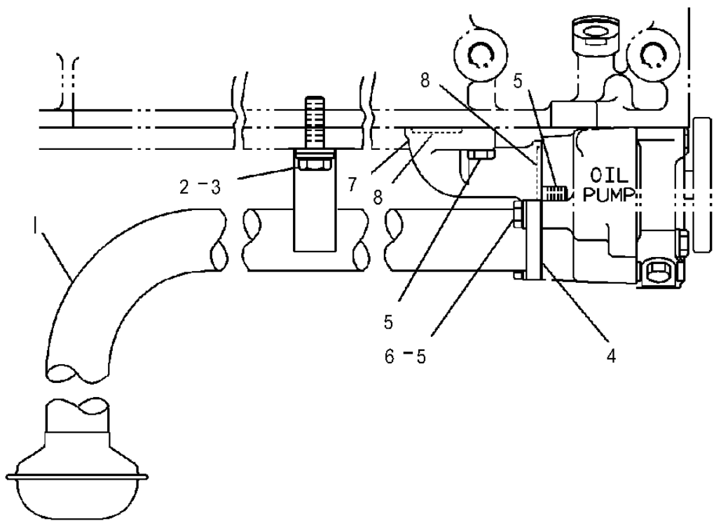
SIDE VIEW
