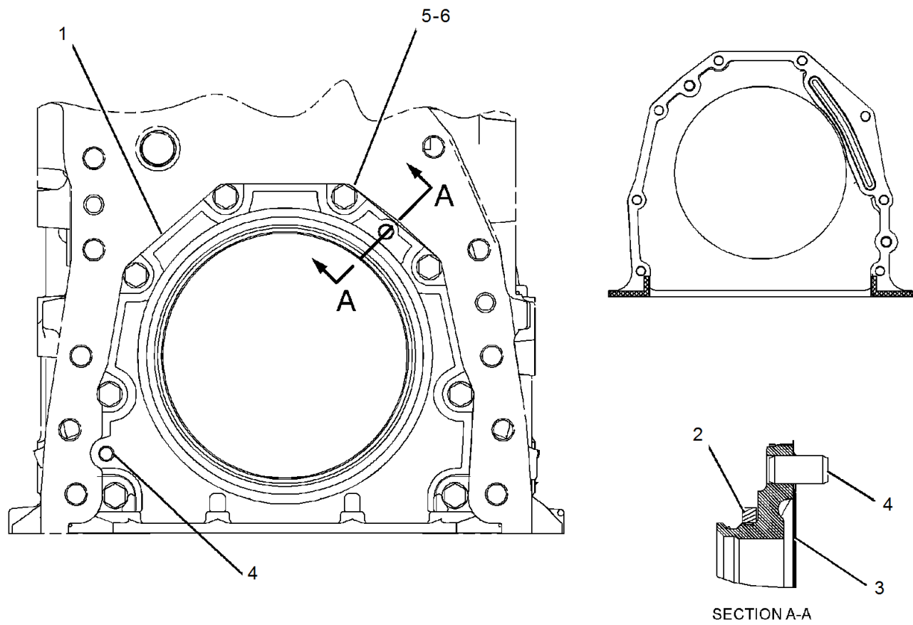
Drawing 1 of 1
