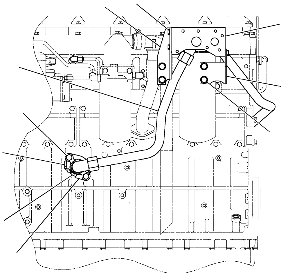
LEFT SIDE VIEW OF ENGINE
