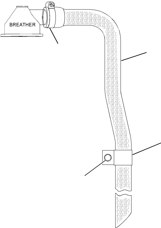
FRONT SIDE OF ENGINE
