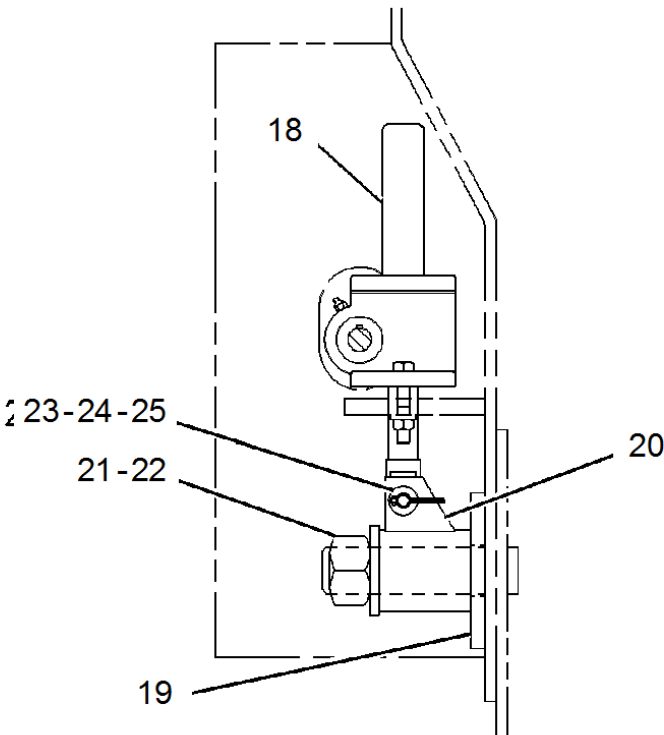
VIEW D-D
