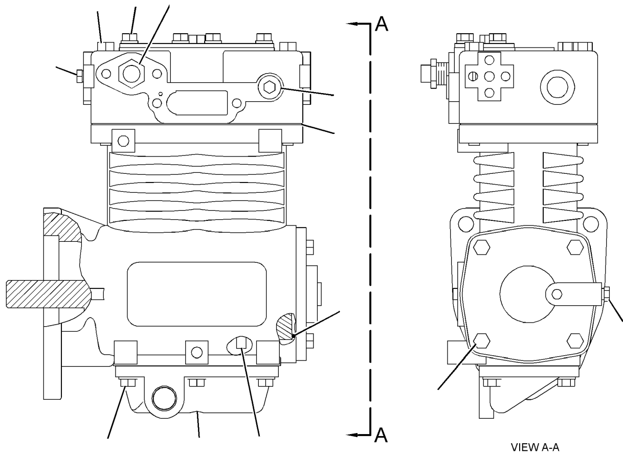
Drawing 1 of 1
