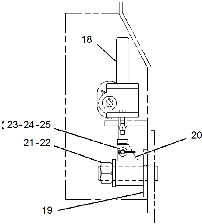
VIEW D-D
