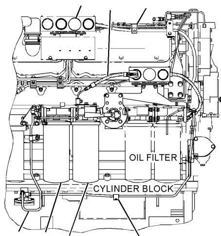
RIGHT SIDE VIEW OF ENGINE
