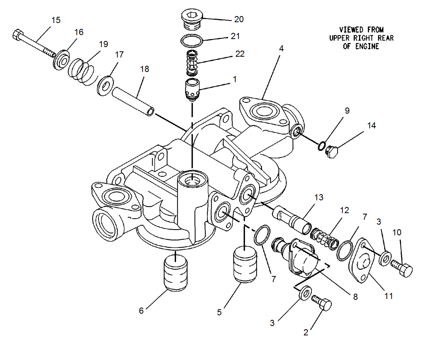
Drawing 1 of 1
