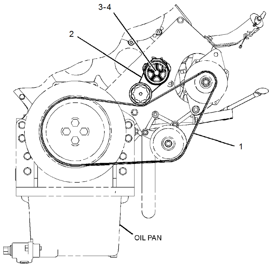
FRONT VIEW
