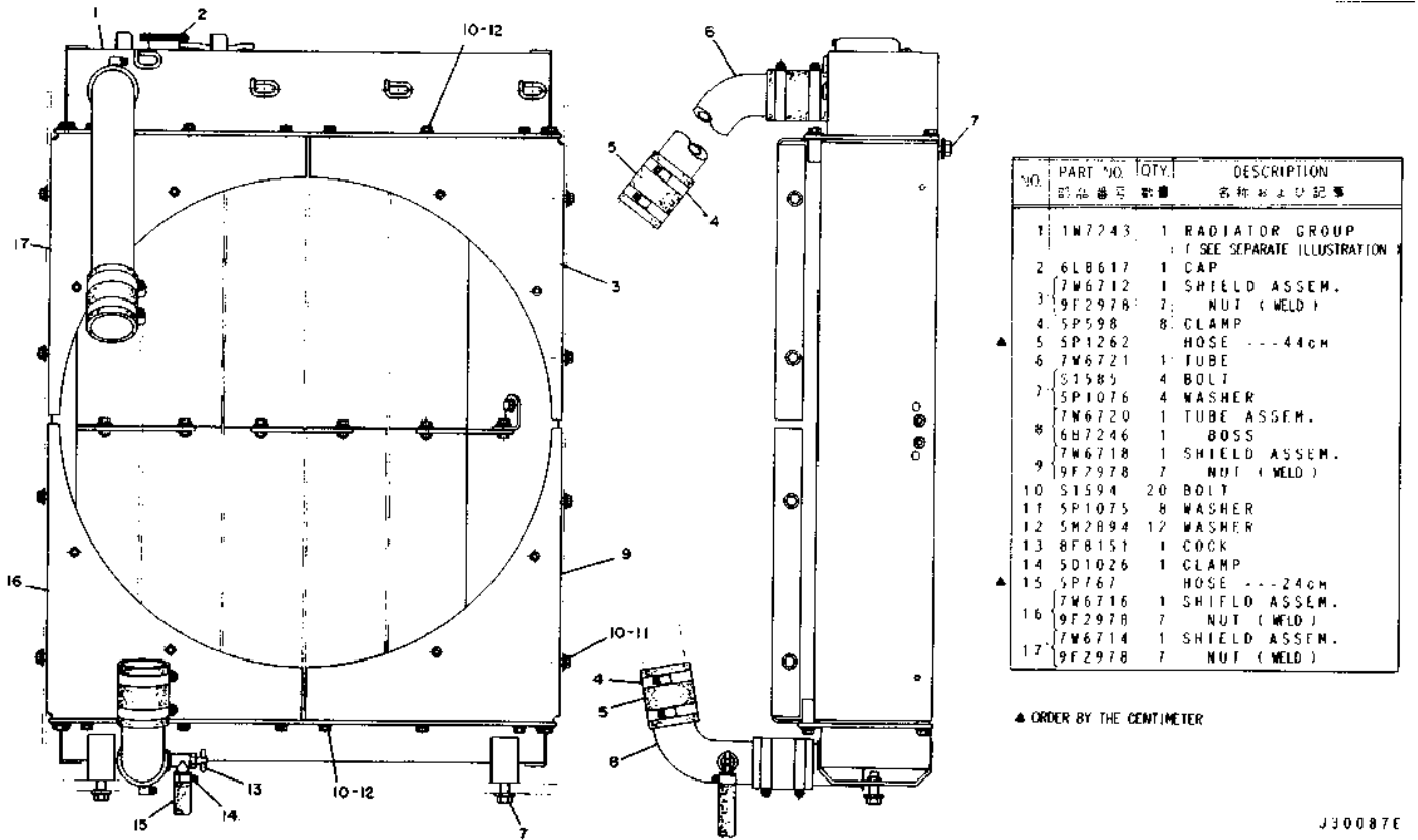
Drawing 1 of 1
