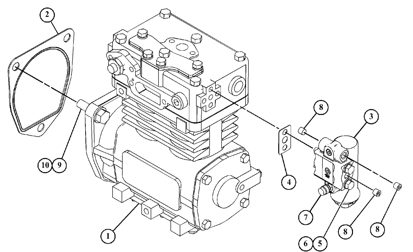
Drawing 1 of 1
