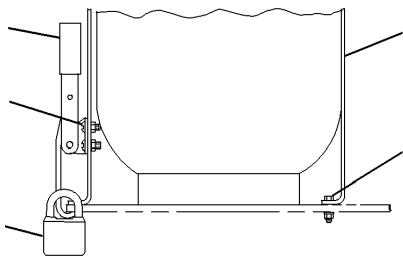
VIEW B-B
