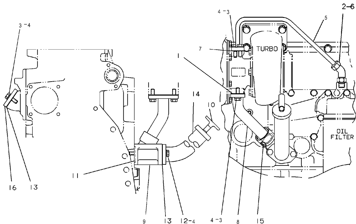
REAR VIEW
