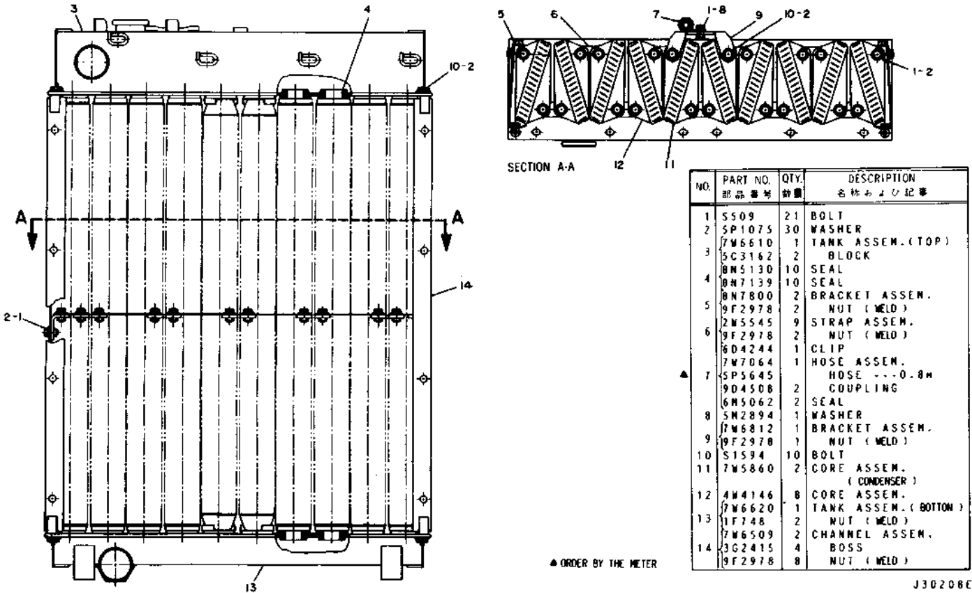
Drawing 1 of 1
