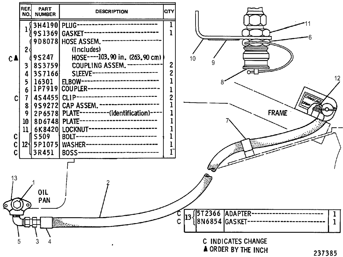
Drawing 1 of 1
