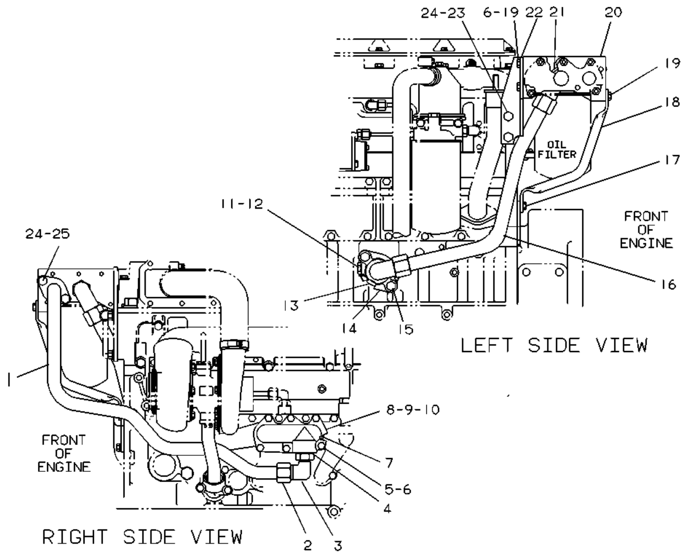
Drawing 1 of 1
