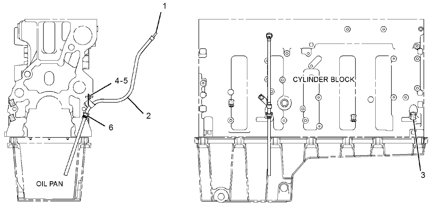
FRONT VIEW OF ENGINE
