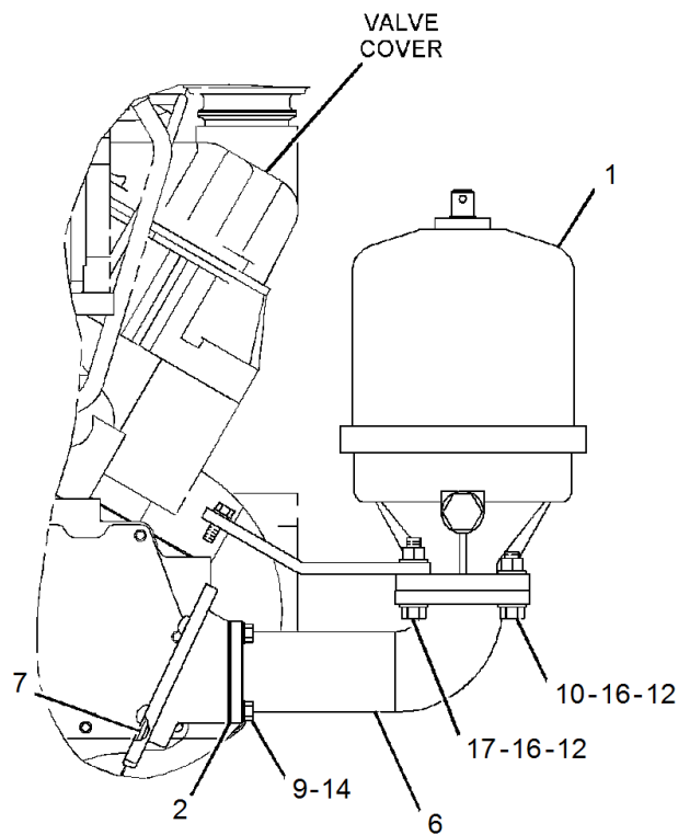
FRONT VIEW OF ENGINE
