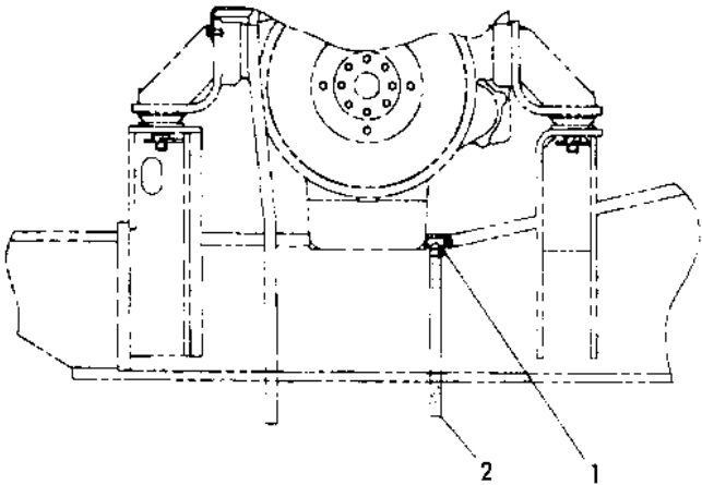
REAR VIEW OF ENGINE
