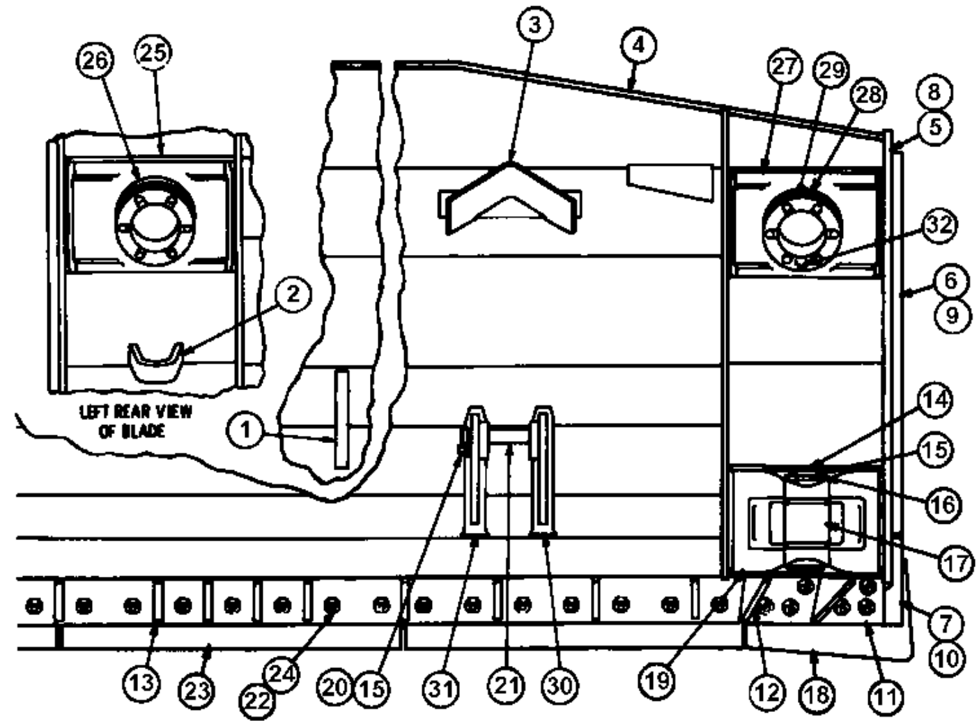
Drawing 1 of 1
