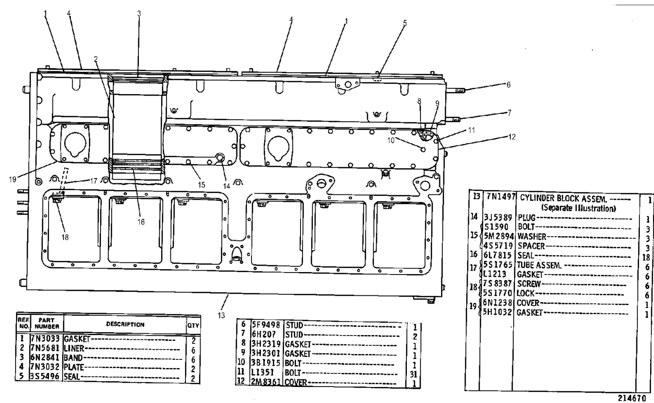
Drawing 1 of 1
