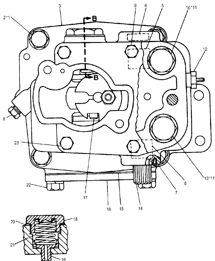
SECTION B-B
