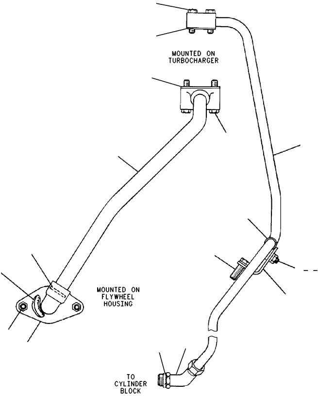
REAR VIEW
